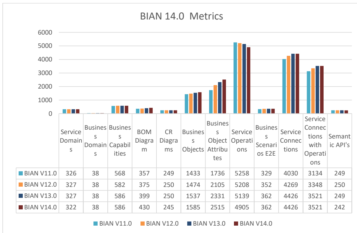
Figure 1 BIAN v14.0 Numbers of artefacts compared to the previous releases
